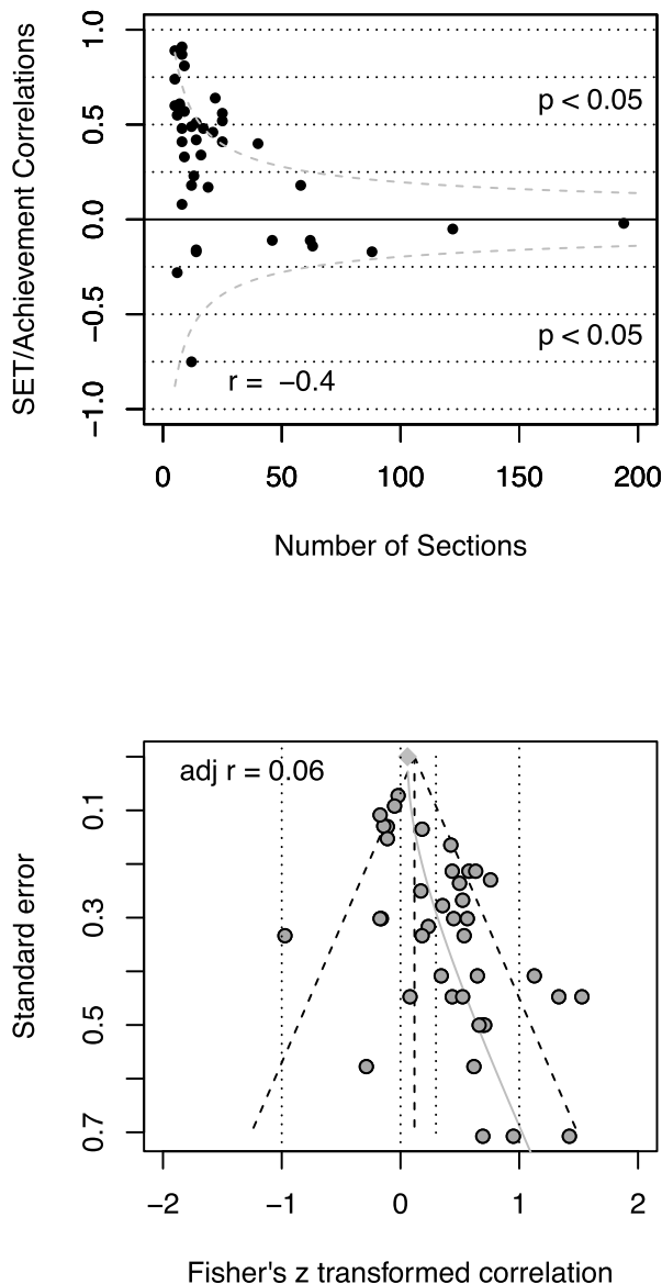
Fig. 4. Re-analysis of Clayson’s (2009) multisection data set. The top left panel shows the small size study effects. The right panel shows cumulative meta-analysis showing that the meta-analysis of large sized studies reveals minimal and negative SET/learning correlation and that addition of smaller size studies increases the estimated SET/learning correlation. The bottom left panel shows the result of limit meta-analysis taking into account small size study effects, including adjusted r = .06 .
