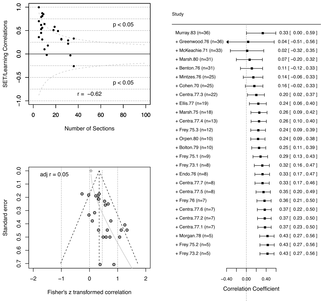
Fig. 3. Re-analysis of Feldman's (1989) multisection data set for Feldman's Dimension 5: Preparation and Organization. The top left panel shows the small size study effects. The right panel shows cumulative meta-analysis showing that the meta-analysis of large sized studies reveal small SET/learning correlation and that addition of smaller size studies increases the estimated SET/learning correlation. The bottom left panel shows the result of limit meta-analysis taking into account small size study effects, including adjusted r = .05 .
