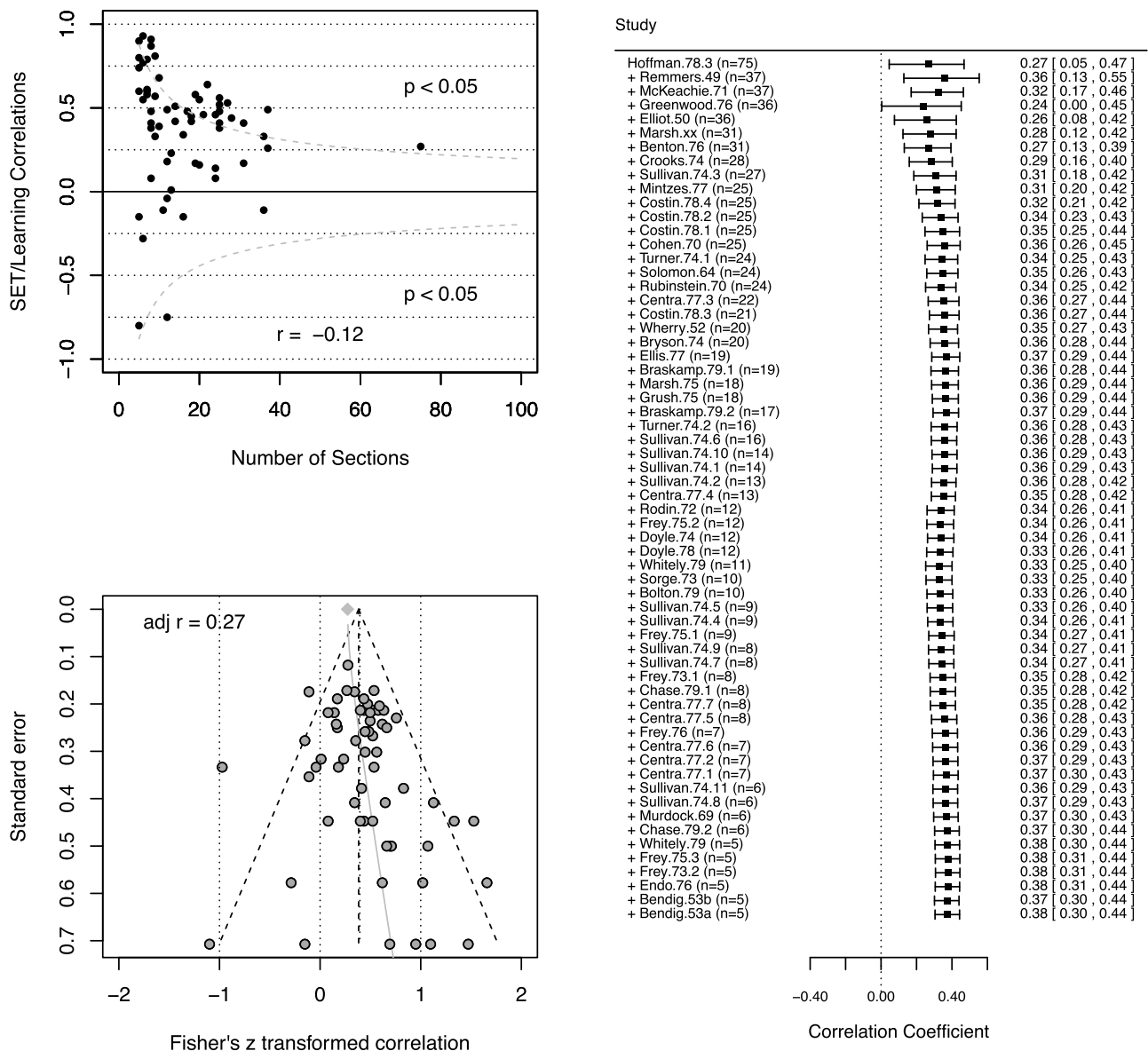
Fig. 2. Re-analysis of Cohen's (1981) multisection data set. The top left panel shows the small size study effects. The right panel shows cumulative meta-analysis showing that the meta-analysis of large sized studies reveals small SET/learning correlation and that addition of smaller size studies increases estimated SET/learning correlation. The bottom left panel shows the result of limit meta-analysis taking into account small size study effects, including adjusted r = .27 .
