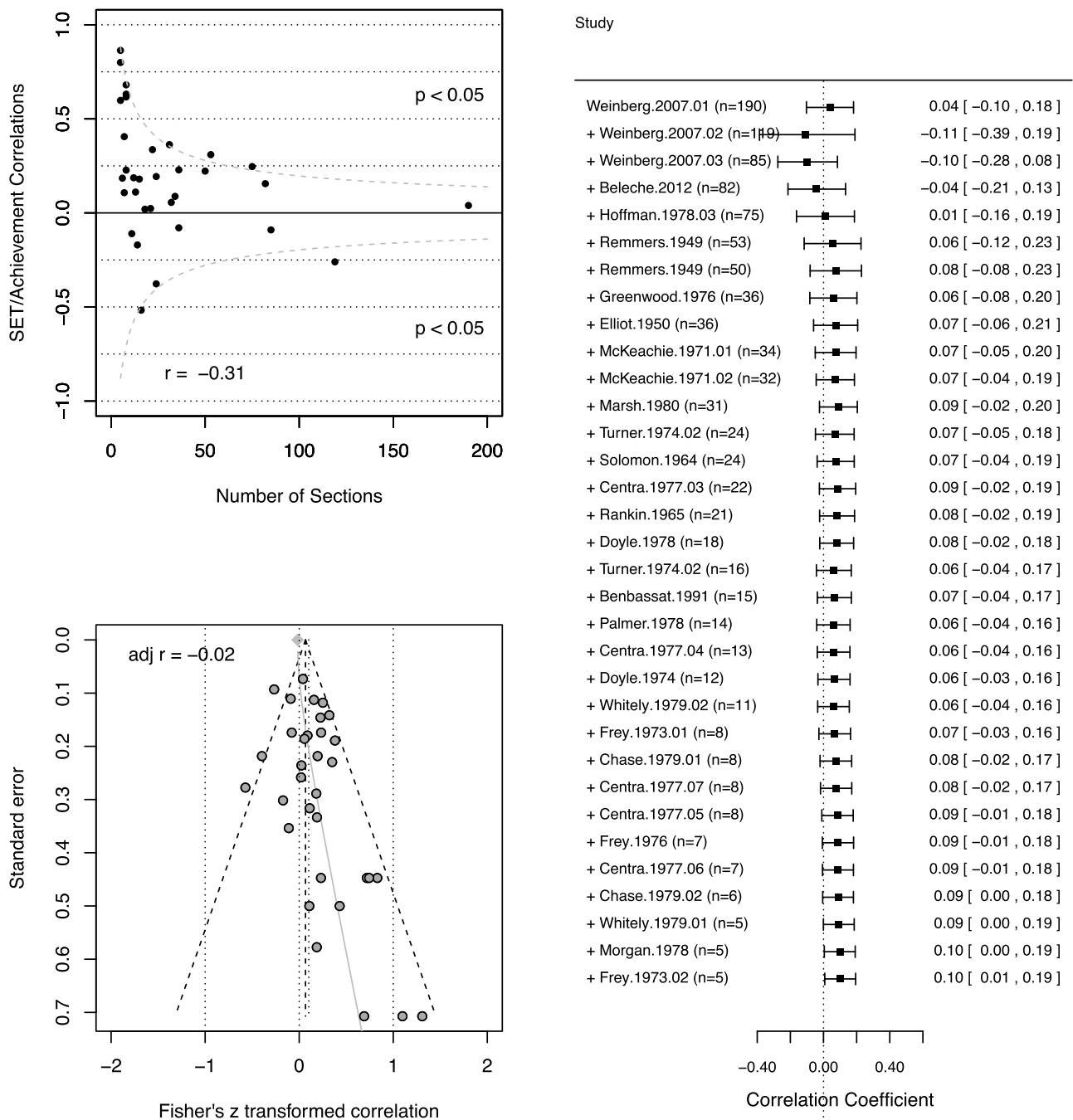
Fig. 10. Meta-analysis of Averaged SET/learning correlations using only correlations adjusted for prior learning/ability. The top left panel shows the small size study effects. The right panel shows cumulative meta-analysis showing that the meta-analysis of large sized studies reveals minimal and nonsignificant SET/learning correlation and that addition of smaller size studies increases estimated SET/learning correlation. The bottom left panel shows the result of limit meta-analysis taking into account small size study effects, including adjusted r = -.02 .
