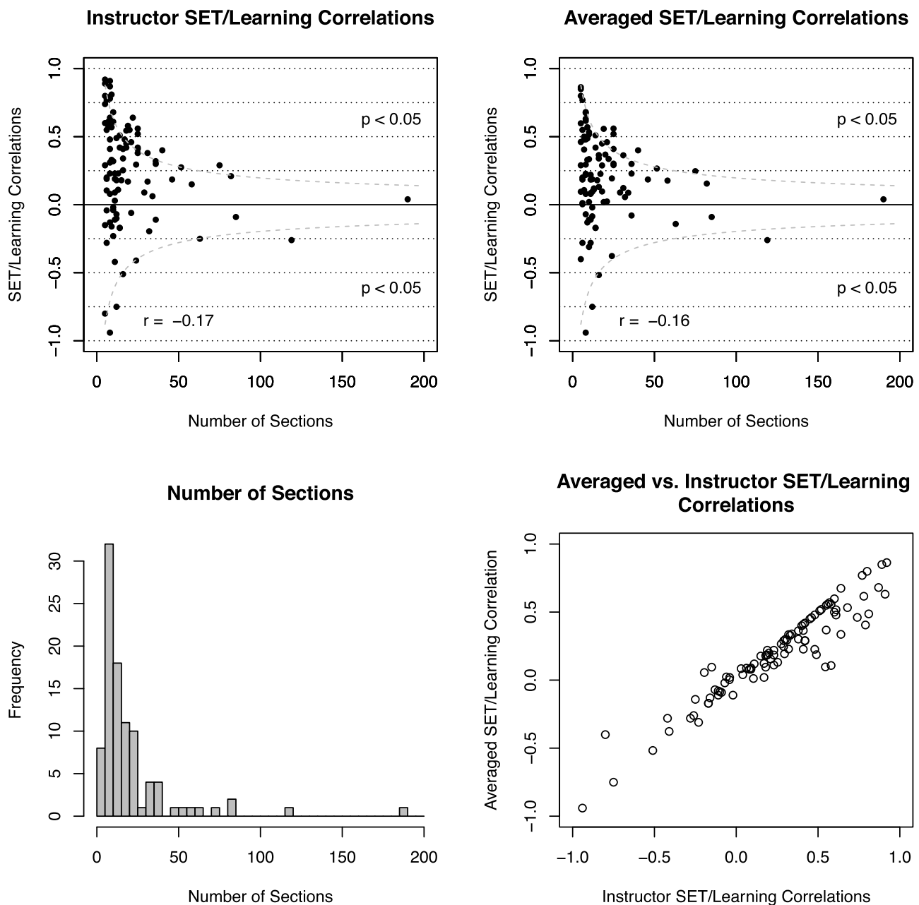
Fig. 6. The top left panel shows the relationship between Instructor SET/learning correlations and study size (number of sections). The top right panel shows the relationship between averaged SET/learning correlations and study size (number of sections). The bottom left panel shows the histogram of the number of sections. The bottom right panel shows the scatterplot between Averaged vs. Instructor SET/learning correlations ( r = .95 ).
