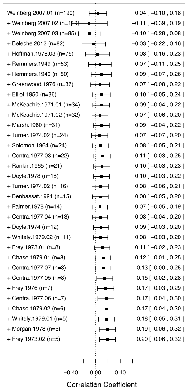
Fig. 8. Meta-analysis of Instructor SET/learning correlations using only correlations adjusted for prior learning/ability. The top left panel shows the small size study effects. The right panel shows cumulative meta-analysis showing that the meta-analysis of large sized studies (i.e., with > 30 sections) suggests minimal and non significant SET/learning correlation and that addition of smaller size studies increases the estimated SET/learning correlation. The bottom left panel shows the result of limit meta analysis taking into account small size study effects, including adjusted r = -.04 .
